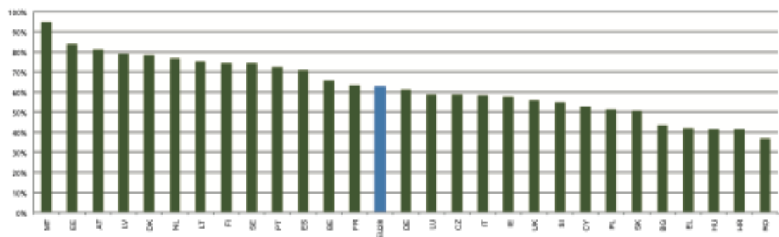
Figure 8.4: Digitisation Index
